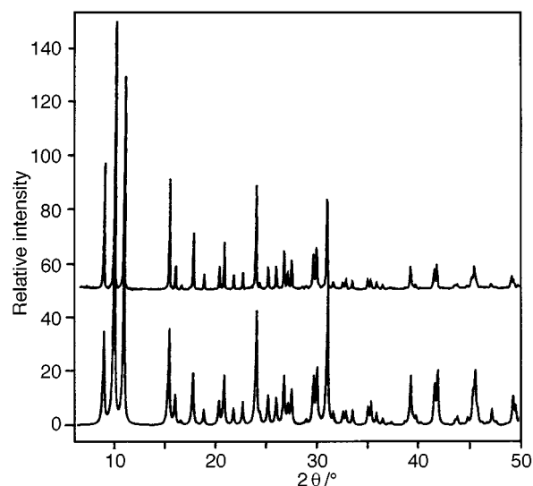
Fig. 3 X-Ray powder pattern for (TMA) 4 Ge 4 Se 10 (top) compared with the simulated powder pattern (bottom) from single-crystal data, created by CERIUS ® software
