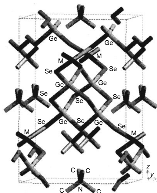
Fig. 4 A CERIUStm molecular graphics representation of (TMA) 2 MGe 4 Se 10 showing the adamantanoid Ge 4 X 10 4- and M 2+ on alternate tetrahedral sites of a zinc-blende lattice. The TMA + charge balancing cations occupy the void space of the open framework structure (hydrogen atoms are omitted for clarity)
