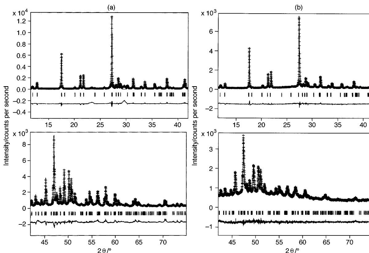
Fig. 1 Observed (+, I_o ), calculated (-, I_c ) and difference ( I_o - I_c ) high resolution room-temperature PXRD patterns of (a) (\text{TMA})_2\text{MnGe}_4\text{Se}_{10} and (b) (\text{TMA})_2\text{FeGe}_4\text{Se}_{10}
